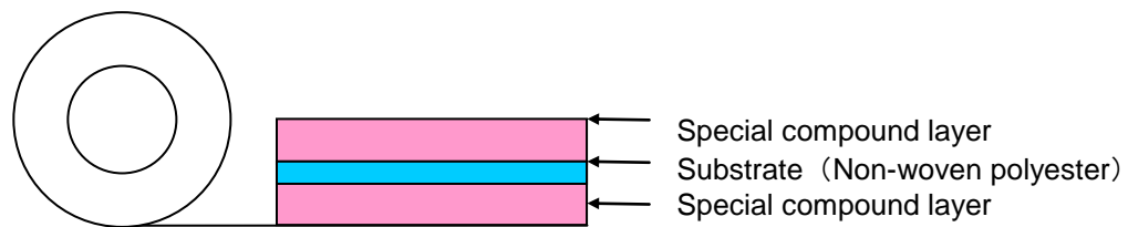
Fig1. Tape structure
